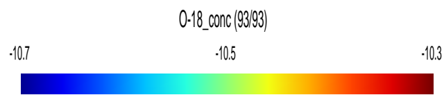
Figure 5.7: Transport of isotopes in two-dimensional model.
