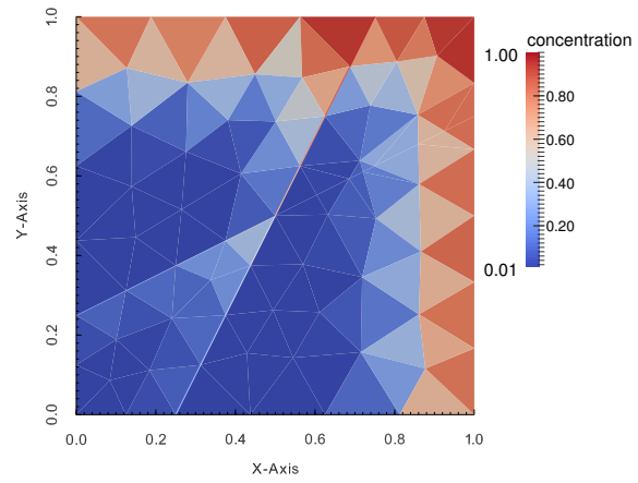
(b) Propagation of U235 from the inflow part of the boundary. (At the time 9 \cdot 10^5 s.)
